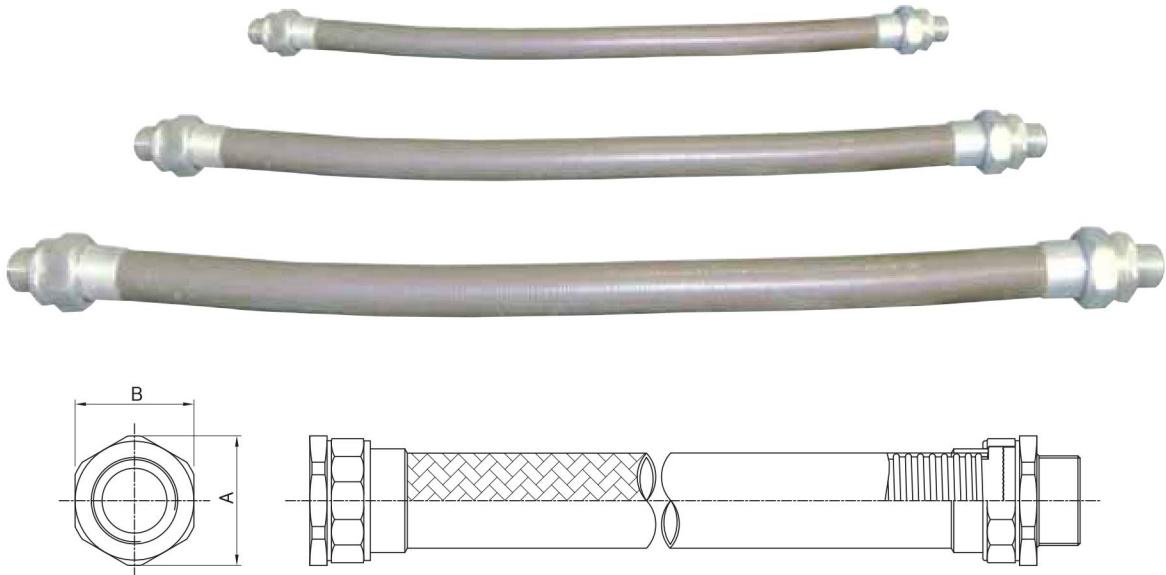
Type of Explosion-Proof Increased safety proof (Ex e II)
