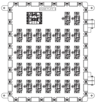
30 CKT'S
