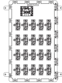
20 CKT'S
