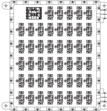
40 CKT'S
