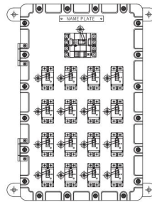
16 CKT'S
