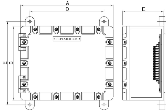
Type of Explosion-Proof Flameproof (Ex d IIB+H2 T6)
